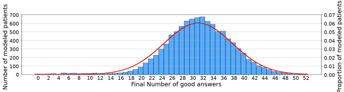
Figure 8: Frequency of good answers over 10,000 runs (in blue) and its fitting normal distribution with \mu = 31.2131 and \sigma^2 = 43.9271 (in red).
