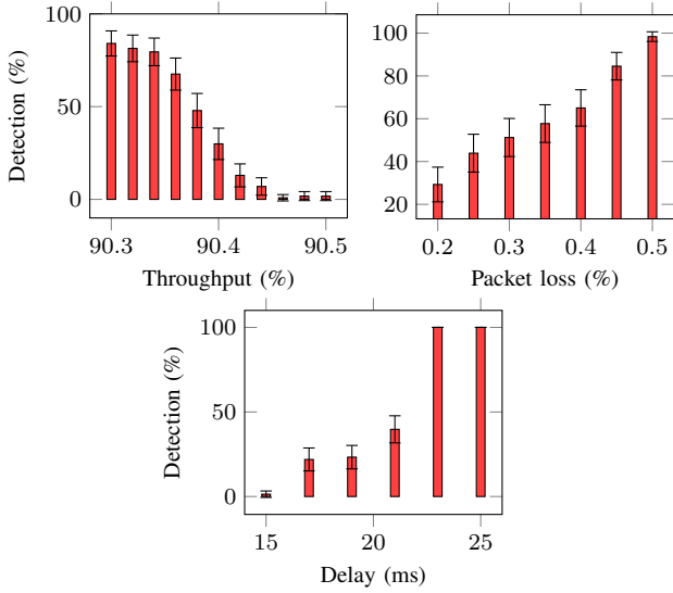
Fig. 2. Wehe detection probability estimations in the case of file transfer for three types of differentiation, with 95% confidence intervals
