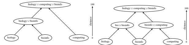
(a) A classical dendrogram, hiding the early relationship between bioinfo and computing . (b) A quasi-dendrogram, preserving the relationships of bioinfo .
