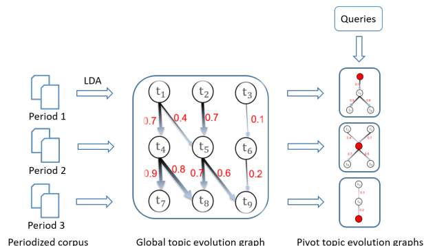
Figure 1: Topic evolution model of EPIQUE
