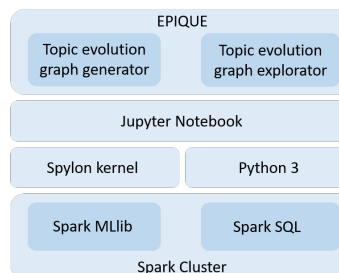
Figure 2: EPIQUE web application architecture
