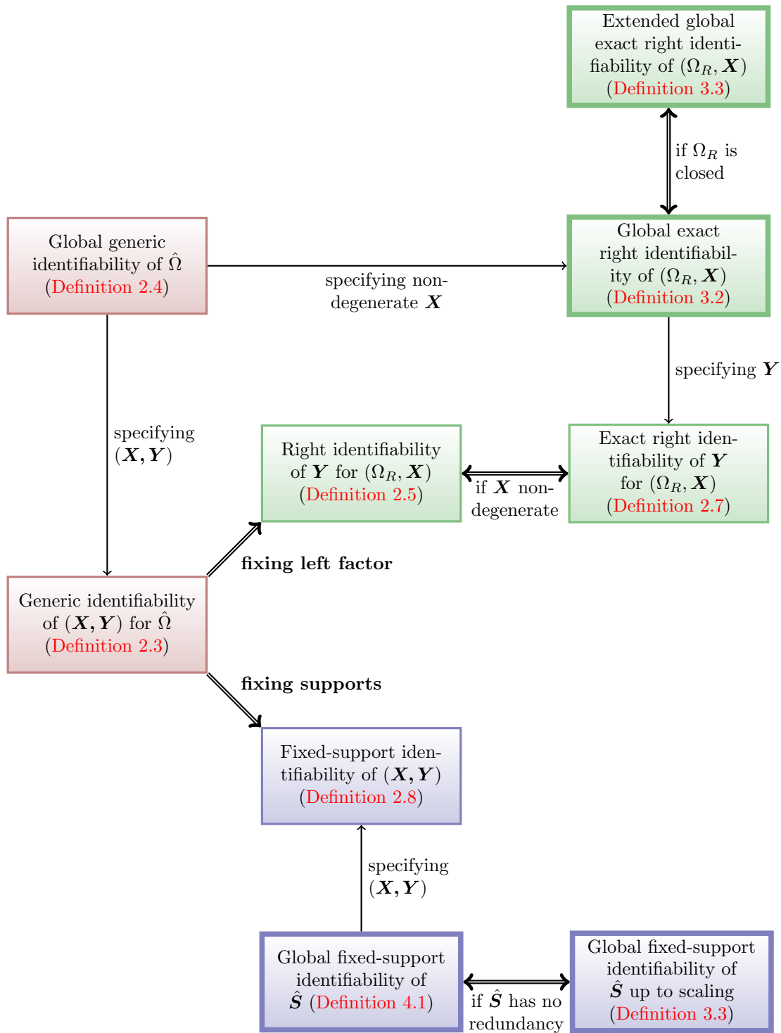
Figure 2.1: Relation between different notions of identifiability introduced in this work. Each box color corresponds to a specific problem: red for the generic problem (Problem 1), green for the problem variation where the left factor is fixed (Problem 2), and blue for the problem variation where the pair of supports is fixed (Problem 3). Thick boxes correspond to notions of identifiability that have been characterized in this work.
