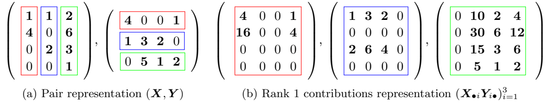
Figure 4.1: Example of rank 1 contribution representations for a pair of factors (\mathbf{X}, \mathbf{Y}) \in \mathbb{C}^{4 \times 3} \times \mathbb{C}^{3 \times 4} . Nonzero entries are represented in bold.
