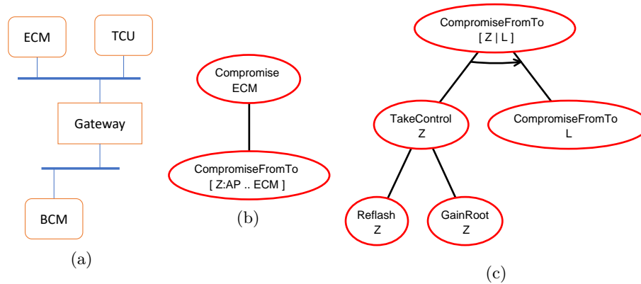
Fig. 4. The compromise attack template tree.
