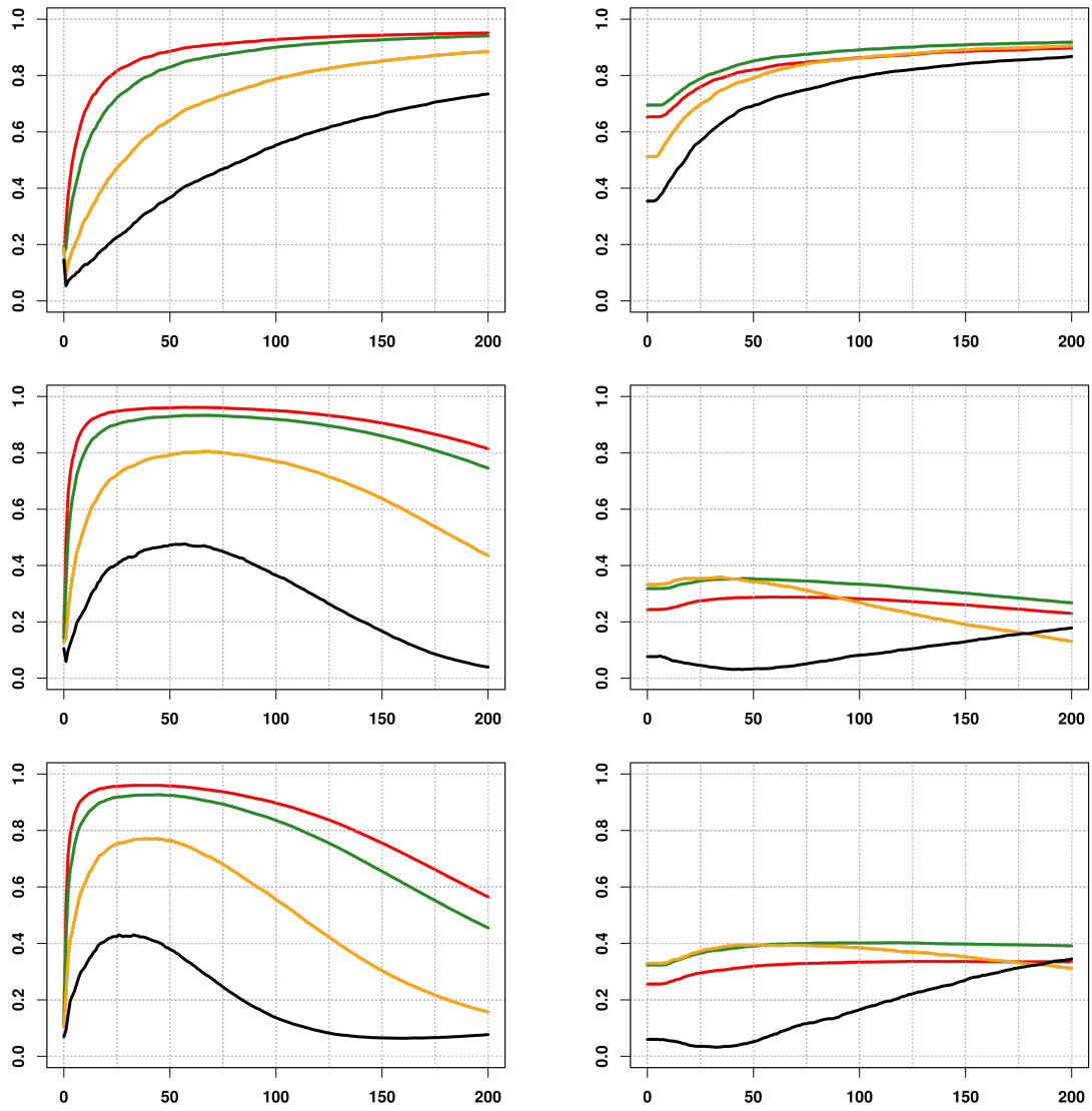
Fig. A.3: Finite sample behaviour of EPLS \hat{v}(Y_{n-k+1,n}) (left) and SIMEXQ (right) estimators, on simulated data from a Student distribution, Frank copula, dimension p = 30 . Horizontally: number k \in \{1, \dots, 200\} of exceedances, vertically: PC(Y_{n-k+1,n}) quality measure. From top to bottom, Frank copula parameter \theta \in \{0, 10, 20\} . The powers c \in \{1/4, 1/2, 1, 3/2\} of the link function g(t) = t^c are displayed in {black, yellow, green, red}.
