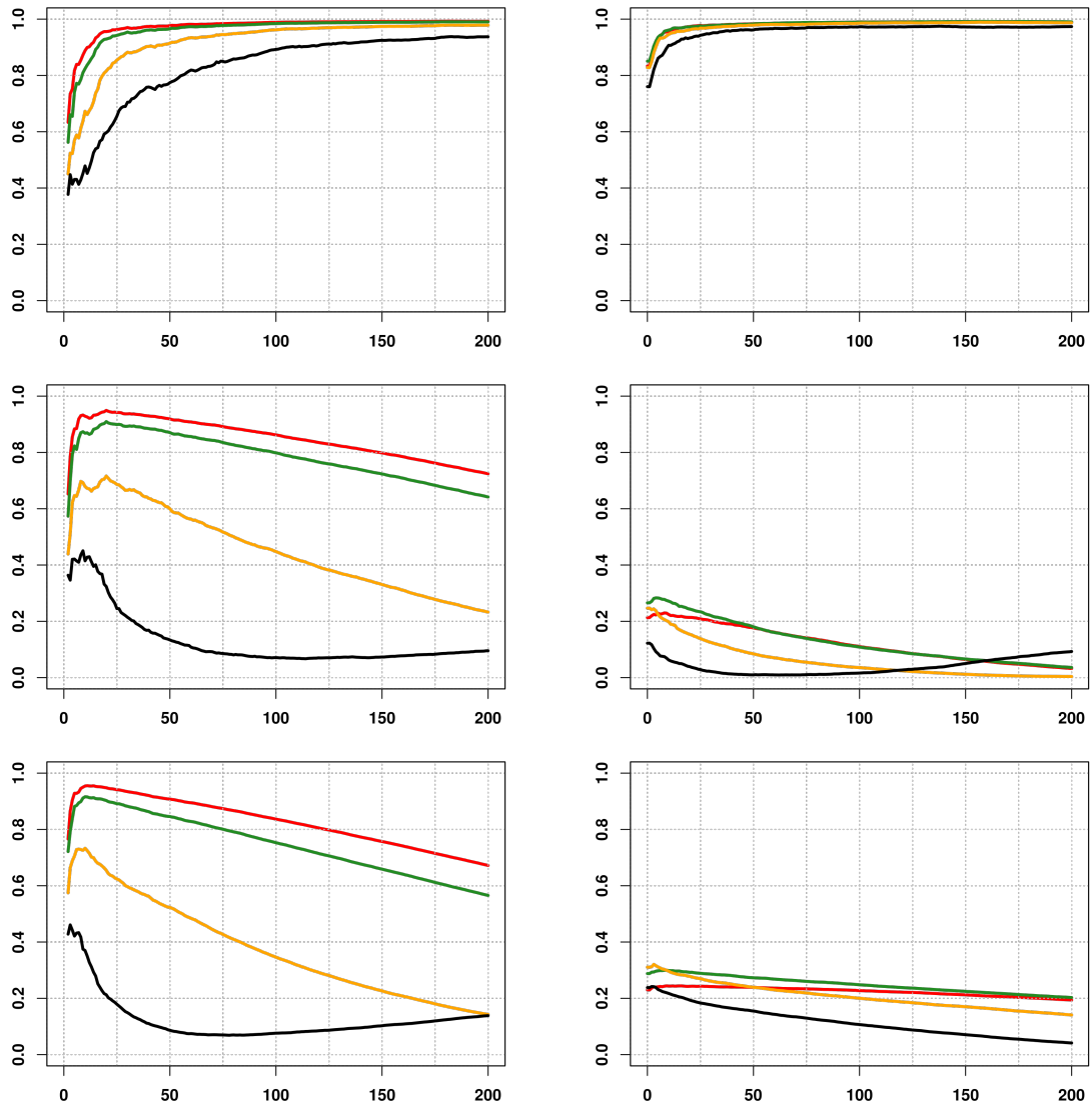
Fig. A.4: Finite sample behaviour of EPLS \hat{\nu}(Y_{n-k+1,n}) (left) and SIMEXQ (right) estimators, on simulated data from a Pareto distribution, Gaussian copula, dimension p = 3 . Horizontally: number k \in \{1, \dots, 200\} of exceedances, vertically: PC(Y_{n-k+1,n}) quality measure. From top to bottom, Gaussian copula parameter \theta \in \{0, 0.87, 0.96\} . The powers c \in \{1/4, 1/2, 1, 3/2\} of the link function g(t) = t^c are displayed in {black, yellow, green, red}.
