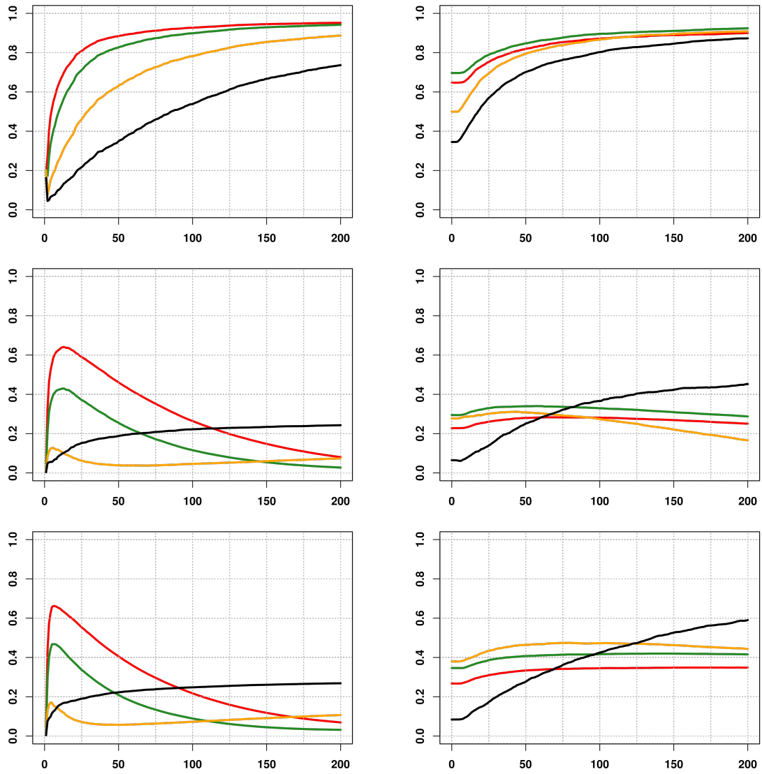
Fig. A.7: Finite sample behaviour of EPLS \hat{\nu}(Y_{n-k+1,n}) (left) and SIMEXQ (right) estimators, on simulated data from a Student distribution, Gaussian copula, dimension p = 30 . Horizontally: number k \in \{1, \dots, 200\} of exceedances, vertically: PC(Y_{n-k+1,n}) quality measure. From top to bottom, Gaussian copula parameter \theta \in \{0, 0.87, 0.96\} . The powers c \in \{1/4, 1/2, 1, 3/2\} of the link function g(t) = t^c are displayed in {black, yellow, green, red}.
