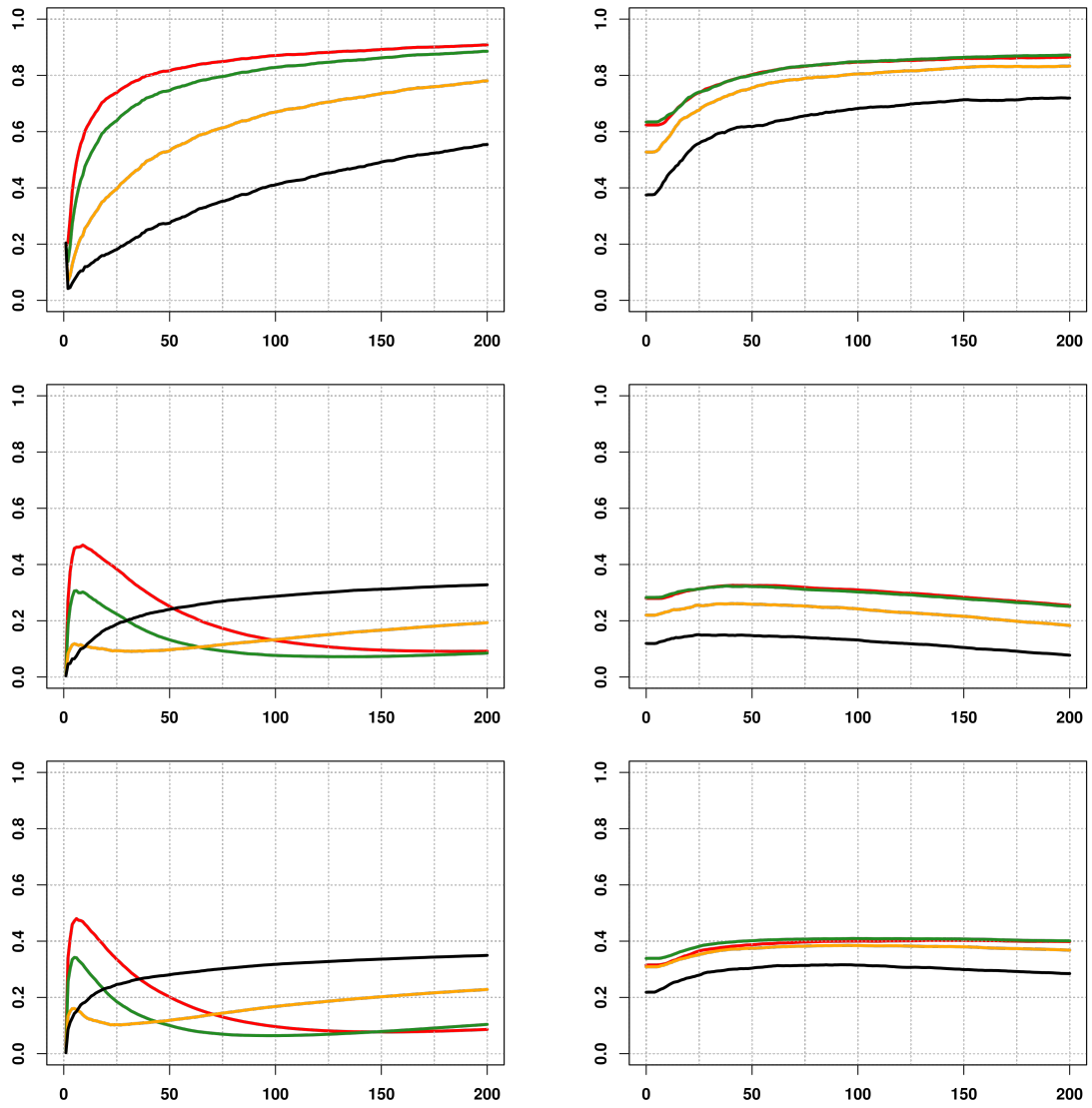
Fig. A.6: Finite sample behaviour of EPLS \hat{\nu}(Y_{n-k+1,n}) (left) and SIMEXQ (right) estimators, on simulated data from a Pareto distribution, Gaussian copula, dimension p = 30 . Horizontally: number k \in \{1, \dots, 200\} of exceedances, vertically: PC(Y_{n-k+1,n}) quality measure. From top to bottom, Gaussian copula parameter \theta \in \{0, 0.87, 0.96\} . The powers c \in \{1/4, 1/2, 1, 3/2\} of the link function g(t) = t^c are displayed in {black, yellow, green, red}.
