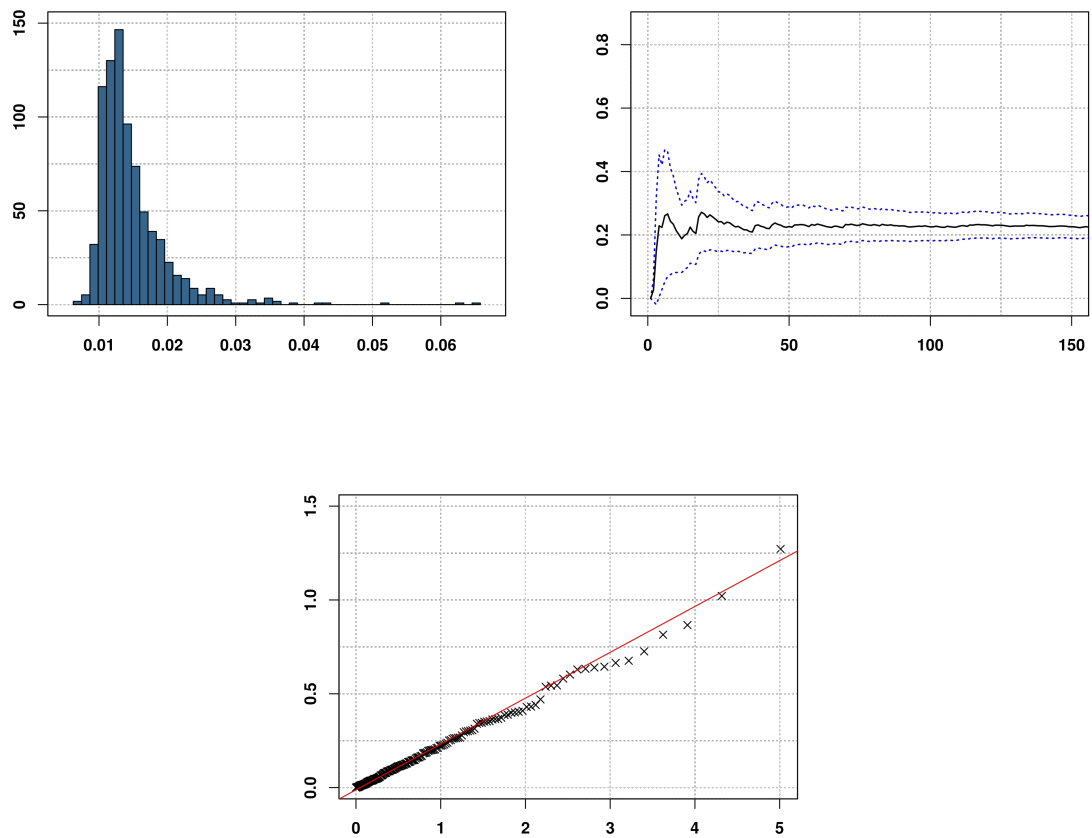
Fig. 3: Farm income data. Top left panel: Histogram of the inverse yields Y_i , i = 1, \dots, n . Top right panel: Hill plot (Horizontally: k \in \{1, \dots, 150\} , vertically: Hill estimator \hat{\gamma}_k , dashed blue line: empirical 95% confidence interval). Bottom panel: quantile-quantile plot (horizontally: \log(k/i) , vertically: \log(Y_{n-i+1,n}/Y_{n-k,n}) for i \in \{1, \dots, k = 150\} , red: regression line).
