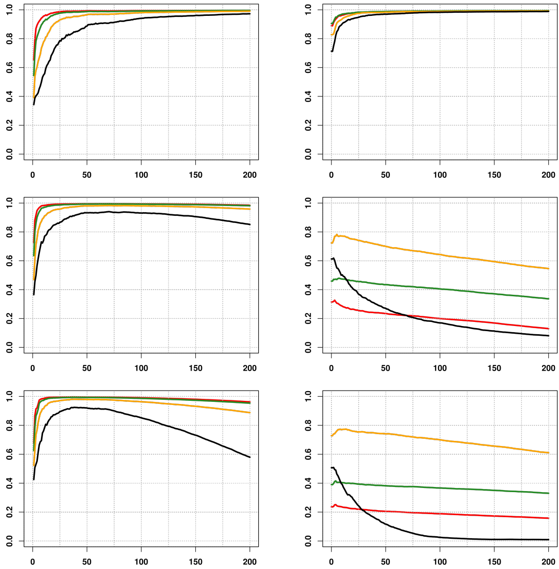
Fig. A.1: Finite sample behaviour of EPLS \hat{v}(Y_{n-k+1,n}) (left) and SIMEXQ (right) estimators, on simulated data from a Student distribution, Frank copula, dimension p = 3 . Horizontally: number k \in \{1, \dots, 200\} of exceedances, vertically: PC(Y_{n-k+1,n}) quality measure. From top to bottom, Frank copula parameter \theta \in \{0, 10, 20\} . The powers c \in \{1/4, 1/2, 1, 3/2\} of the link function g(t) = t^c are displayed in {black, yellow, green, red}.
