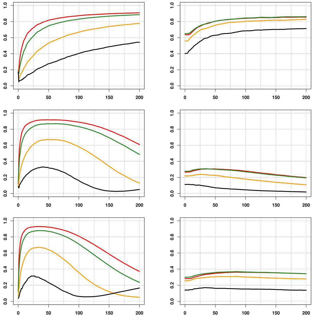
Fig. A.2: Finite sample behaviour of EPLS \hat{v}(Y_{n-k+1,n}) (left) and SIMEXQ (right) estimators, on simulated data from a Pareto distribution, Frank copula, dimension p = 30 . Horizontally: number k \in \{1, \dots, 200\} of exceedances, vertically: PC(Y_{n-k+1,n}) quality measure. From top to bottom, Frank copula parameter \theta \in \{0, 10, 20\} . The powers c \in \{1/4, 1/2, 1, 3/2\} of the link function g(t) = t^c are displayed in {black, yellow, green, red}.
