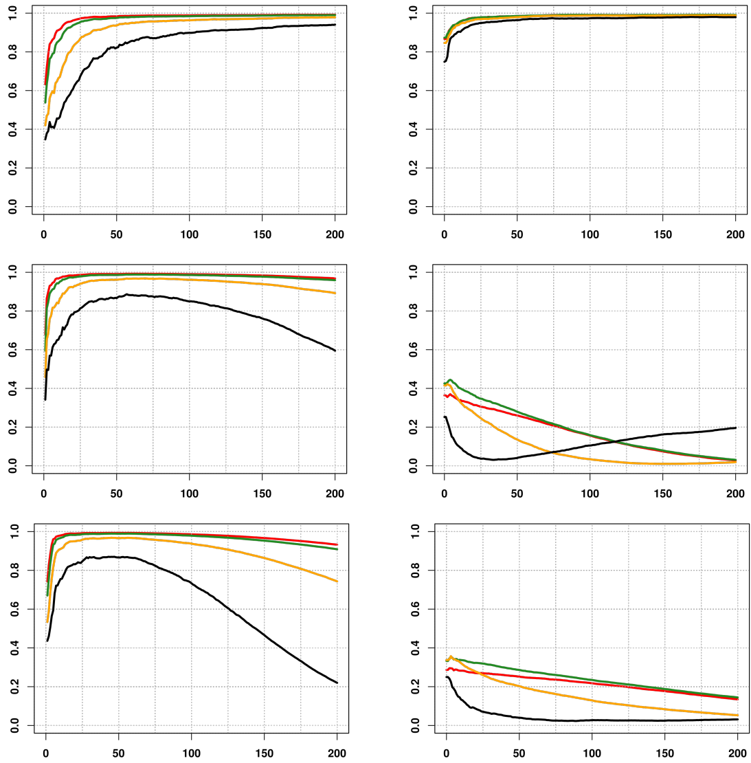
Fig. 2: Finite sample behaviour of EPLS \hat{\nu}(Y_{n-k+1,n}) (left) and SIMEXQ [56] (right) estimators, on simulated data from a Pareto distribution, Frank copula, dimension p = 3 . Horizontally: number k \in \{1, \dots, 200\} of exceedances, vertically: PC(Y_{n-k+1,n}) quality measure. From top to bottom, Frank copula parameter \theta \in \{0, 10, 20\} . The powers c \in \{1/4, 1/2, 1, 3/2\} of the link function g(t) = t^c are displayed in {black, yellow, green, red}.
