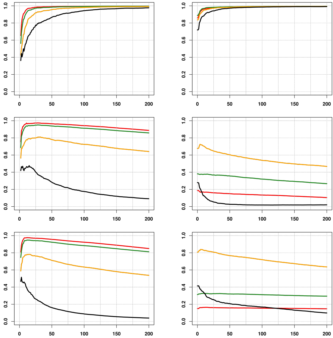
Fig. A.5: Finite sample behaviour of EPLS \hat{v}(Y_{n-k+1,n}) (left) and SIMEXQ (right) estimators, on simulated data from a Student distribution, Gaussian copula, dimension p = 3 . Horizontally: number k \in \{1, \dots, 200\} of exceedances, vertically: PC(Y_{n-k+1,n}) quality measure. From top to bottom, Gaussian copula parameter \theta \in \{0, 0.87, 0.96\} . The powers c \in \{1/4, 1/2, 1, 3/2\} of the link function g(t) = t^c are displayed in {black, yellow, green, red}.
