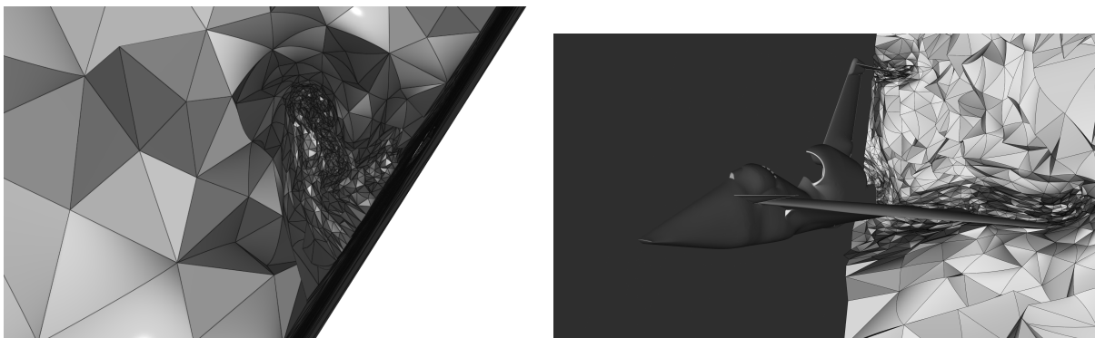
Fig. 16 Turbulent wake of the supersonic aircraft (front and rear view). Edge curvature is visible curling along with the vortex.
