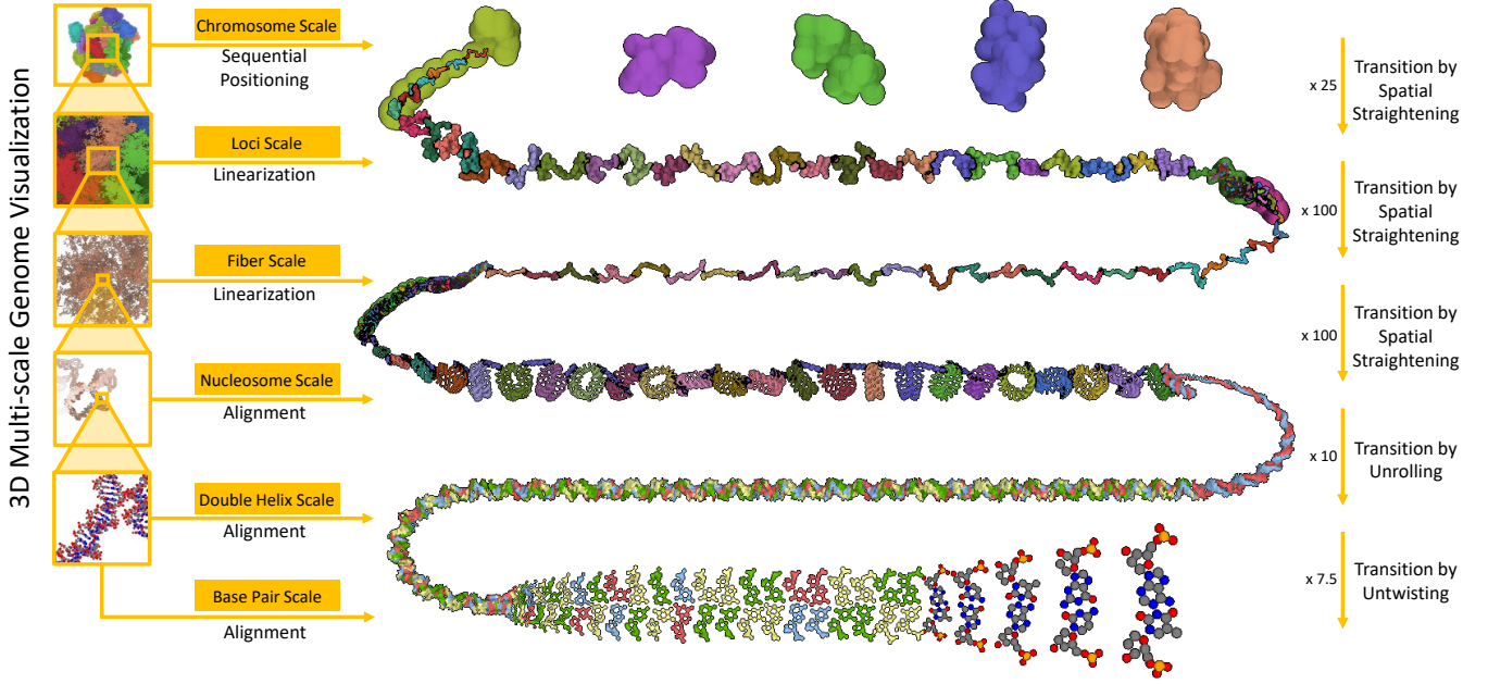
Fig. 1. Multiscale unfolding with continuous scale transitions of the 3D human genome, showing chromosomes, loci, fibers, nucleosomes, double helix, and flattened base pairs. Scales 1–4 are composed of details from the next-lower scale, and linearized based on the elements' own positions.
