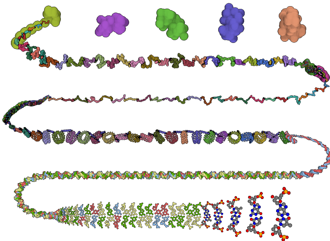
Fig. 12. Large version of the multiscale unfolding zig-zag layout in Fig. 1.
