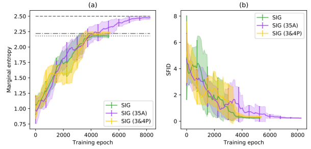
Figure 6: Effects of increasing the size of action dictionary (SIG (35A)) and adding four-people interactions to the original three-people interaction dataset (SIG (3&4P)) on marginal entropy (a) and SFID (b). Standard model is shown for comparison. All models were trained on sequences of 40 actions with \lambda_{sup} = 0 . Gray dashed, dash-dotted and dotted lines represent respectively real data marginal entropy for large dictionary, three and four-people interactions and original SocialInteractionGAN experiments.
