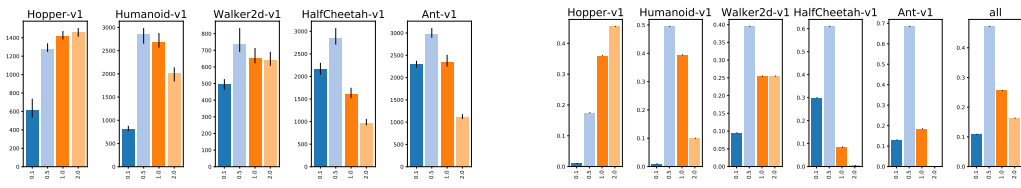
Figure 28: Analysis of choice Initial standard deviation i_\rho (C61): 95th percentile of performance scores conditioned on choice (left) and distribution of choices in top 5% of configurations (right).
