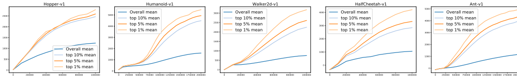
Figure 39: Training curves.
