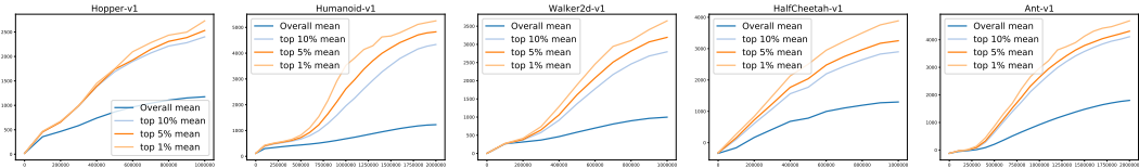
Figure 31: Training curves.
