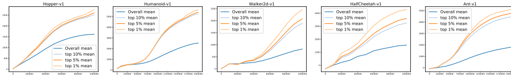
Figure 75: Training curves.
