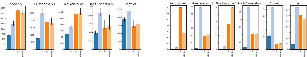
Figure 47: Analysis of choice N-step N (C7): 95th percentile of performance scores conditioned on sub-choice (left) and distribution of sub-choices in top 5% of configurations (right).
