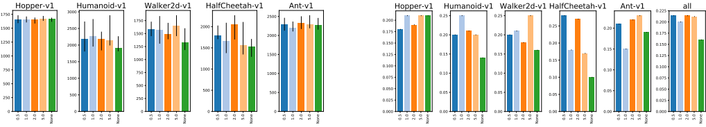
Figure 34: Analysis of choice Gradient clipping (C68): 95th percentile of performance scores conditioned on choice (left) and distribution of choices in top 5% of configurations (right).
