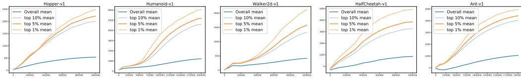
Figure 16: Training curves.
