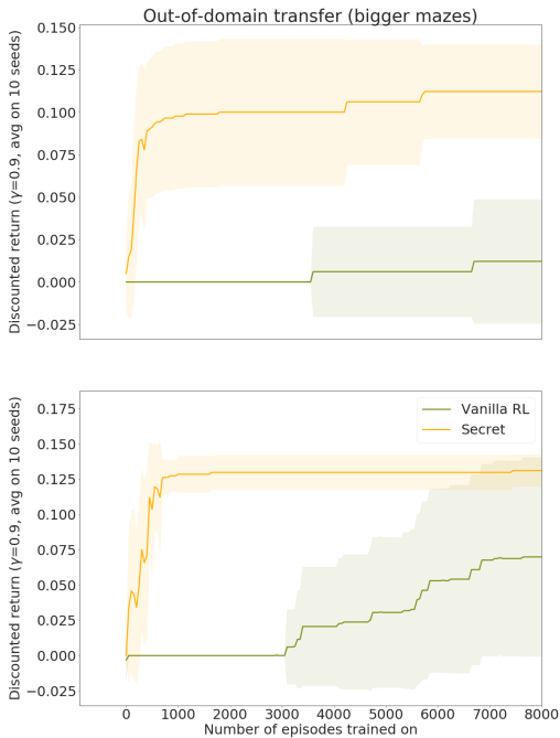
Figure 5: Bigger environments we consider are bigger mazes where the structure of the original task is conserved (number of triggers, number of prizes). Environments drawn are 12x12 grids with 1 trigger and 1 prize for the top figure versus 2 prizes for the bottom one. Environments from the training distribution are 8x8 grids.
