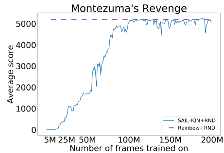
Figure 8: Combining SAIL and RND elevates the performance of IQN and matches that of RND-Rainbow, the best reported in Taiga et al. [42] on Montezuma's Revenge.
