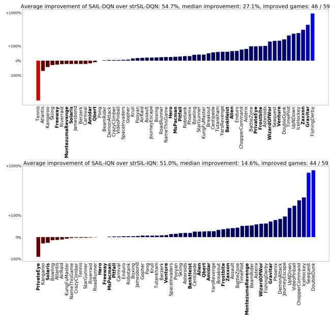
Figure 11: Relative improvement of SAIL over self-imitation (strSIL), based on both DQN (top) and IQN (bottom). On hard exploration games (in bold), SAIL-DQN provides a +72.2% average and +45.2% median relative improvement over strSIL-DQN, and SAIL-IQN a +16.0% average and +22.3% median relative improvement over strSIL-IQN.
