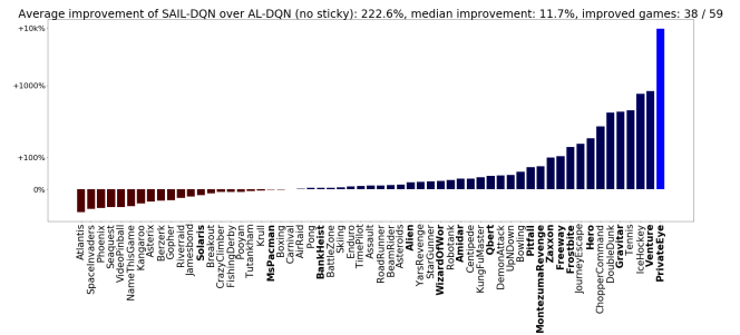
Figure 9: Improvement of SAIL-DQN over AL-DQN on all Atari games, without sticky actions. Result do not diverge from those in the standard ALE setting (+222.6% versus +101.4% average, +11.7% versus +6.7% median).
