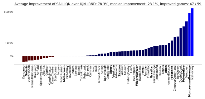
Figure 7: SAIL-IQN outperforms RND-IQN, as shown on a relative scale on all Atari games, including on Montezuma's Revenge, an infamously hard exploration game.
