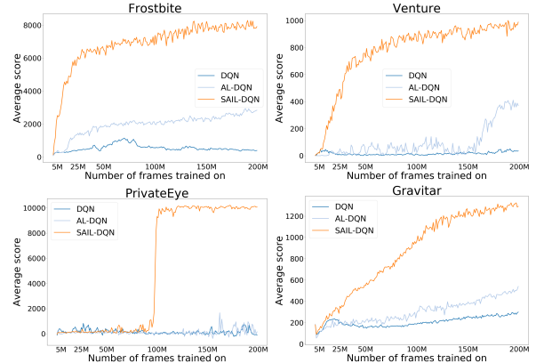
Figure 4: Performances of DQN, AL-DQN and SAIL-DQN on four hard exploration Atari games. On PrivateEye, despite sparse rewards, SAIL-DQN outperforms both C51 and IQN.
