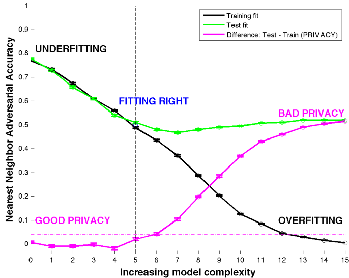
Figure 3: Parzen Windows, learning curves. The Train \mathcal{AA} keeps decreasing, but not the test \mathcal{AA} . The privacy is good when the difference Test \mathcal{AA} - Train \mathcal{AA} is small. The best compromise is attained around the point where the black curve crosses the dashed blue line at 0.5. The pink dashed line shows the difference (Test \mathcal{AA} - Train \mathcal{AA} ).
