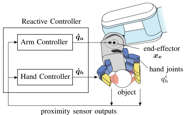
Fig. 16. Reactive control for preshaping is implemented by feeding back the outputs obtained from the proximity sensors mounted on a robot hand, i. e. its palm and fingers, to controllers that affect the pose q_h^i of each finger and the end-effector x_e .
