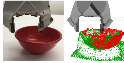
Fig. 18. Complementing a pointcloud obtained by the MS-Kinect with O-ToF sensor inside the gripper PR-2, as shown by Lancaster et al. [128]. (©2017 IEEE)
