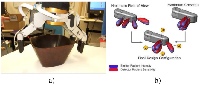
Fig. 10. a) Barrett hand equipped with finger-size optical proximity sensors b) Design criteria leading to a final concept of sensor integration in the fingertips of the Barrett hand. [58] Sensor type: O-RLI (Figures reprinted with kind permission of the authors ©2009 IEEE)
