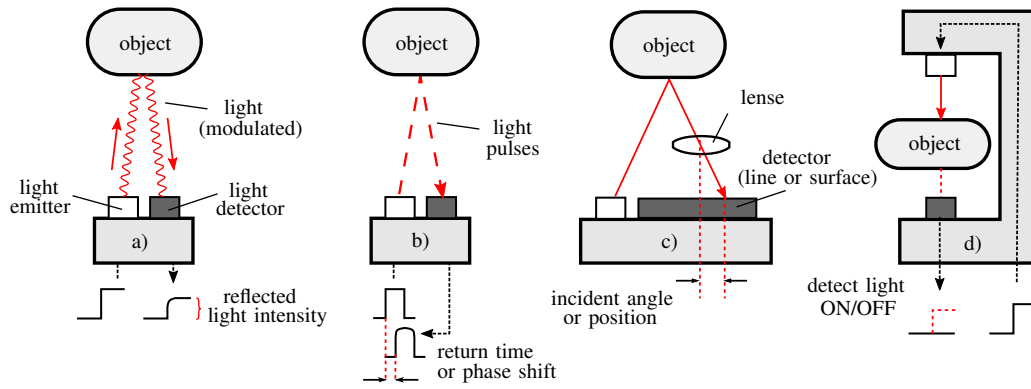
Fig. 8. Illustration of the most common optical sensing working principles: (a) reflected light intensity (O-RLI), (b) time-of-flight (O-ToF), (c) triangulation (O-Tri), and (d) break-beam (O-BB).
