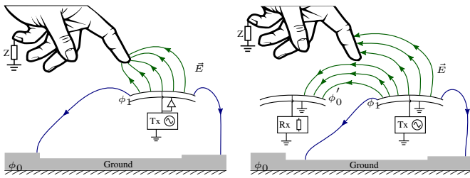
Fig. 6. Capacitive single-ended mode (C-SE) (left): The electrode is driven with an electrical potential and generating an electrical field between the measurement electrode and the object. Mutual-capacitance mode (C-M) (right): the right electrode transmitter (Tx) is driven, generating an electrical field, which ends at receiver (Rx). A conductive object within the measurement range can block/shield the field lines (green) between the electrodes.
