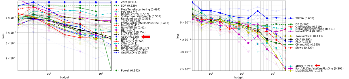
Figure 7: Additional problems (1): on left, Rocket (26 continuous variables, budget up to 1600, sequential or parallelism 30) and on right, SimpleTSP (10 to 1 000 decision variables).
