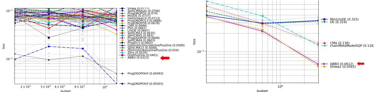
Figure 8: Additional problems (2): on left, PowerSystems (1806 to 9646 neural decision variables) and on right, LSGO (mix of partially separable, overlapping, shifted cases as in [LTO + 13]).
