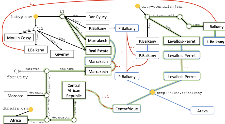
Figure 2: Integrated graph corresponding to the datasets of Figure 1. An answer to the keyword query {“I. Balkany”, Africa, Estate} is highlighted in light green; the labels three keyword matches in this answer are in bold font.
