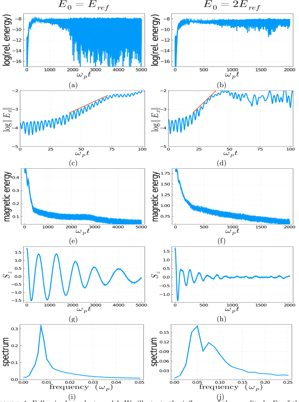
FIGURE 4. Full spin-dependent model. We illustrate the influence of the amplitude E_0 of the incident wave. Left column E_0 = E_{\text{ref}} ; right column E_0 = 2E_{\text{ref}} . First line from top: time history of the the relative total energy |\mathcal{E}_{\text{tot}}(t) - \mathcal{E}_{\text{tot}}(0)|/\mathcal{E}_{\text{tot}}(0) (semi-log e scale). Second line: time history of the longitudinal electric field norm \|E_x\| (semi-log e scale); the red straight lines have slopes 0.03 (left) and 0.06 (right). Third line: magnetic energy \frac{1}{2} \int |B|^2 dx . Fourth line: time history of the spin component S_z(t) . Bottom line: frequency spectrum of S_z .
