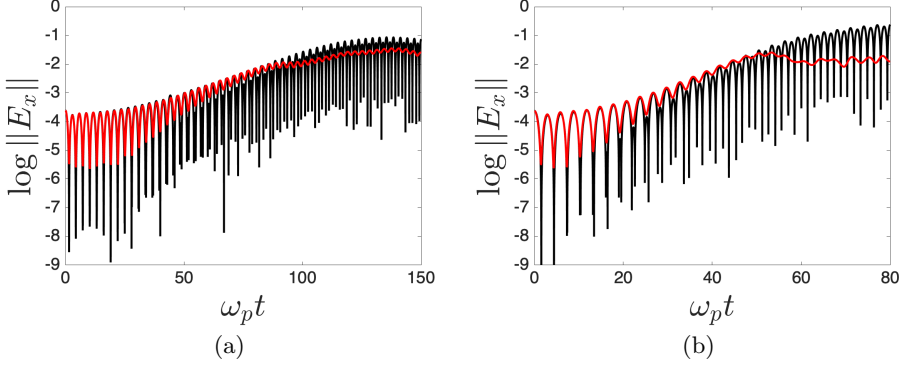
FIGURE 2. SRS simulations without spin. Time evolution of the amplitude of the longitudinal electric field norm \|E_x(t)\| on a semi-log e scale. We compare the results of the Eulerian grid code (black curves) and the PIC code (red curves), for two values of the initial amplitude of the electromagnetic wave. Left frame: E_0 = E_{\text{ref}} = 0.325 (observed slope in the linear regime: \gamma \approx 0.03 ). Right frame: E_0 = 2E_{\text{ref}} = 0.65 ( \gamma \approx 0.06 ).
