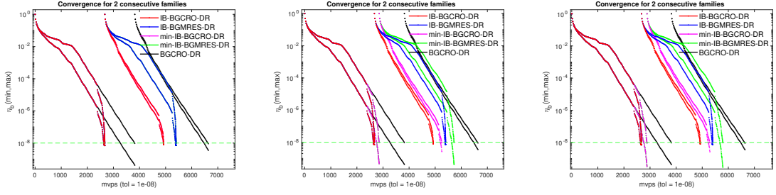
Figure 2: Convergence histories of the largest/smallest backward errors \eta_{b^{(i)}} at each mvps for Section 5.2 with different scaling size of the columns of the RHSs. Comparison the two IB-variants with two different form of IB-threshold by solving Matrix 1 ( p = 20 , m_d = 300 , \varepsilon = 10^{-8} and k = 30 ). Left: B = \text{rand}(n, p) . Middle: B = \text{rand}(n, p) and then multiply 20 to the first \frac{p}{2} columns of B . Right: be the same as the Middle case except for multiplying 50 instead.
