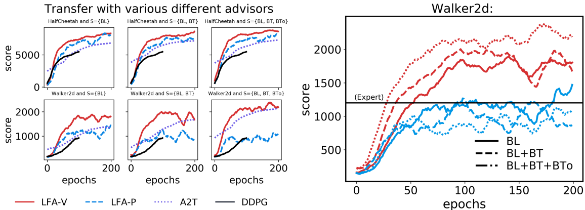
FIGURE 6 – Transfer Learning with several advisors. Figure on the left : Transfer Learning with gradually more advisor provided (increasing from left to right). Figure on the right : Aggregation of the Walker2d results with LEA-V and LEA-P with three settings : one, two and three advisors.
