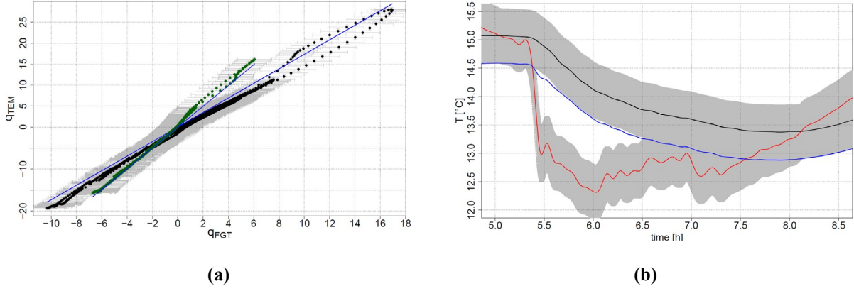
Figure 10. Heat flux measurements from TEM plotted against FGT: (a) q_{b_{TEM}} and q_{b_{FGT}} (black), and q_{s_{TEM}} and q_{s_{FGT}} (green); (b) temperature measurements inside TEM (in black), inside FGT (in blue), and air (in red).
