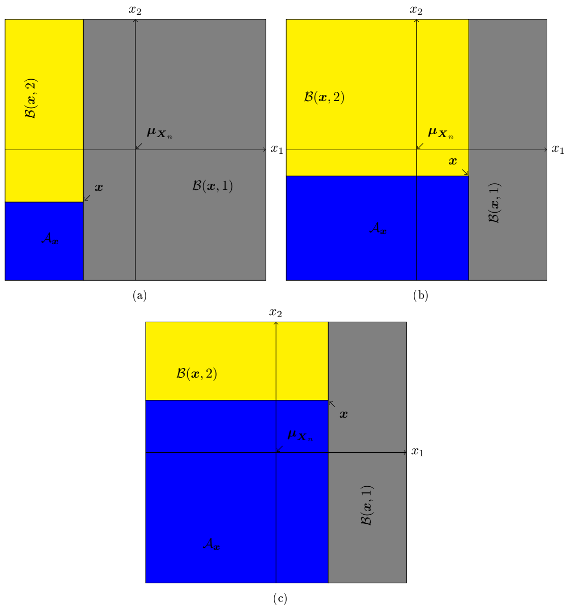
Figure 1: Example of the set \mathcal{A}_{\mathbf{x}} in (34) (blue rectangle); the set \mathcal{B}(\mathbf{x}, 1) (grey rectangle), and the set \mathcal{B}(\mathbf{x}, 2) (yellow rectangle) in (47).
