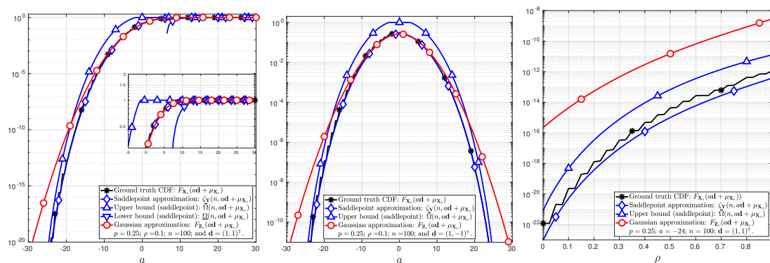
Figure 4: Sum of the independent random vectors \mathbf{Y}_1, \mathbf{Y}_2, \dots, \mathbf{Y}_n , with n = 100 , such that for all i \in \{1, 2, \dots, n\} , \mathbf{Y}_i satisfies (76).
