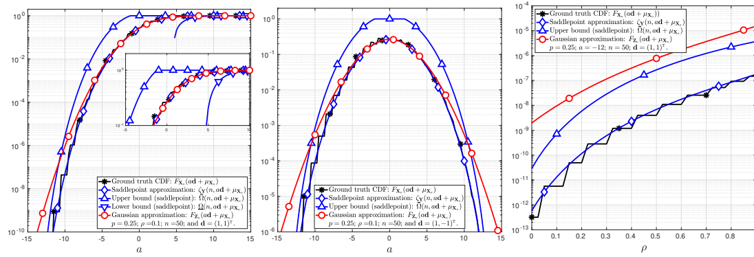
Figure 3: Sum of the independent random vectors \mathbf{Y}_1, \mathbf{Y}_2, \dots, \mathbf{Y}_n , with n = 50 , such that for all i \in \{1, 2, \dots, n\} , \mathbf{Y}_i satisfies (76).
