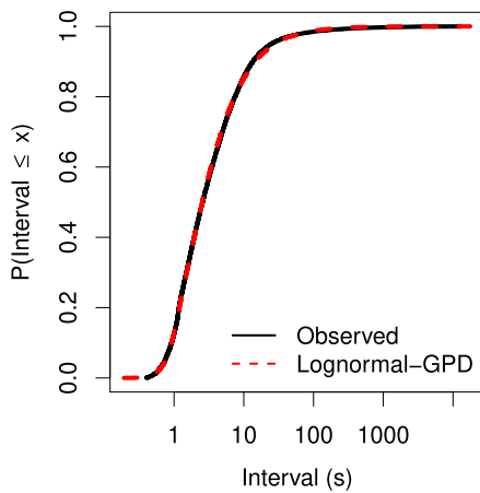
FIGURE 4. CDFs of the user think time according to the empirical data and the best fitted distribution (Lognormal-GPD). The solid line represents the empirical data, while the dashed line represents the fitted distribution.
