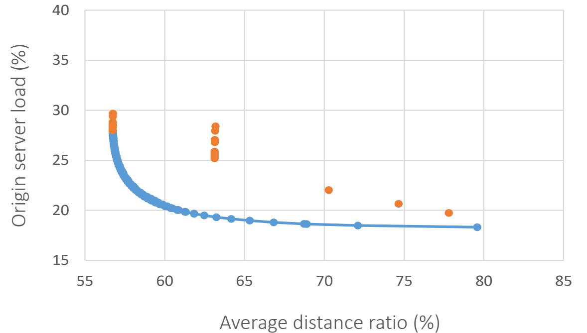
Total cache = 25% / \alpha = 1.0 / 2Q
