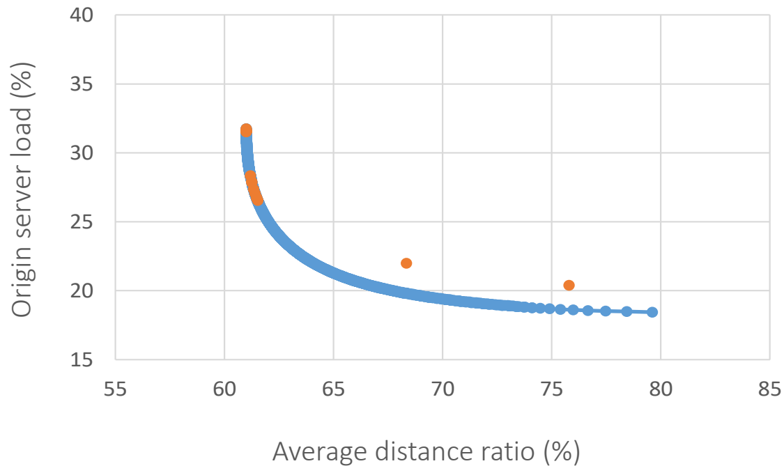
Total cache = 25% / \alpha = 1.0 / LCE
