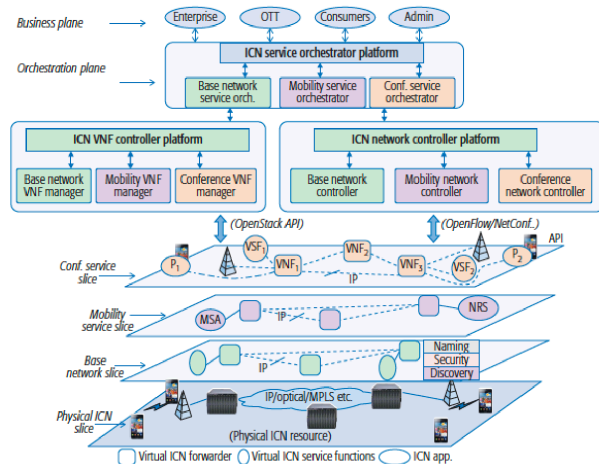
5G ICN Architecture [Ravindran17]
