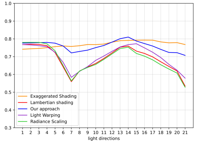
Figure 13: Average congruence scores of previous techniques and our enhancement on the model shown in Figure 14, with 21 different lighting directions (x-axis). A Lambertian shading is used for all the techniques except Exaggerated Shading that relies on its own modified half-Lambertian shading function. The corresponding renderings can be seen in the supplementary document, along with analyses on other scenes.
