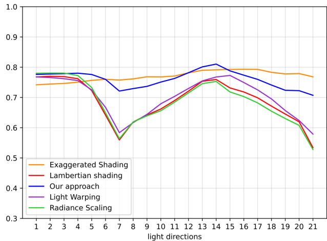
Figure 13: Average congruence scores of previous techniques and our enhancement on the model shown in Figure 14, with 21 different lighting directions (x-axis). A Lambertian shading is used for all the techniques except Exaggerated Shading that relies on its own modified half-Lambertian shading function. The corresponding renderings can be seen in the supplementary document, along with analyses on other scenes.
