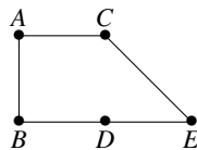
Figure 1: Undirected graph.
