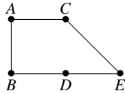
Figure 1: Undirected graph.
