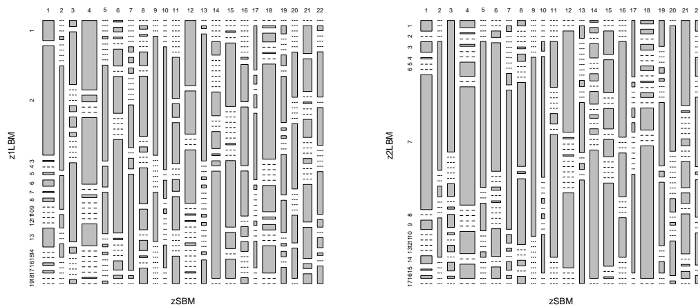
Figure 14: Proportion of row (left) and column (right) LBM clusters in each SBM class.
