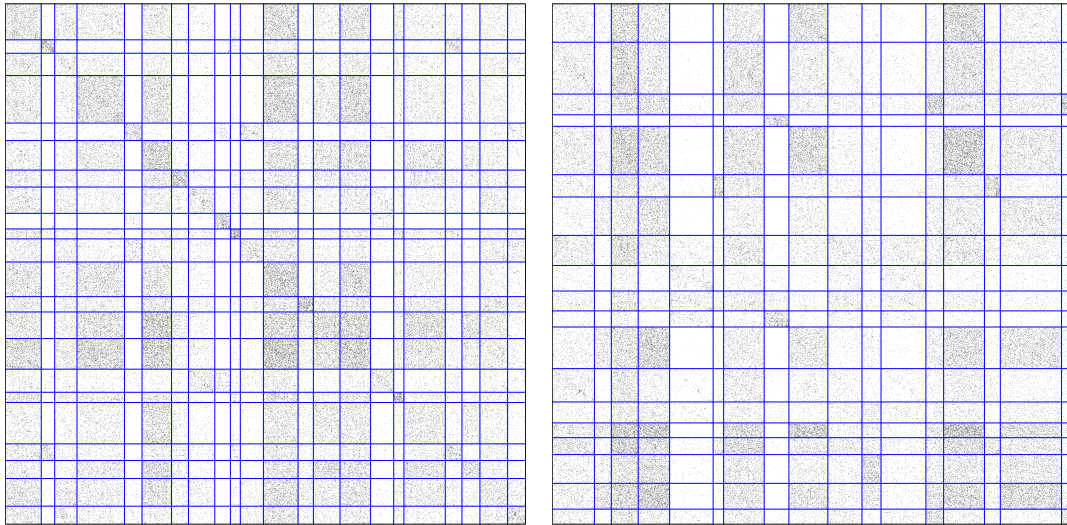
Figure 13: Reorganized adjacency matrices for Arabidopsis data: standard clustering with K = 22 node clusters (left); co-clustering with H = 17 classes of regulated genes (rows) and 19 classes of regulator genes (columns).
