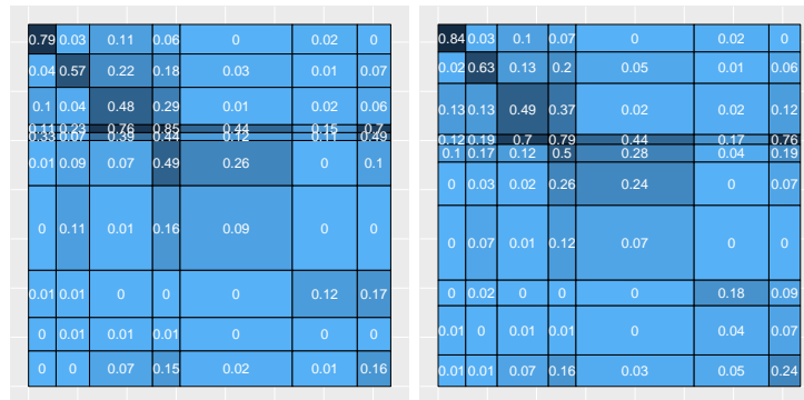
Figure 12: Enron dataset: estimated parameters for SBM after merging the following pairs of column clusters (4,5), (6,7), (8,9) on the left; for LBM on the right.
