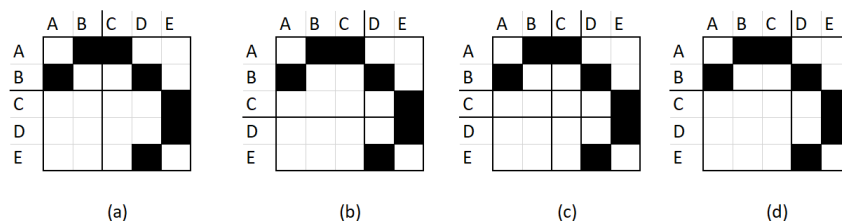
Figure 3: Different clusterings of the directed graph of Figure 2: with the same partition for source and target nodes (a) with the two groups \{(A, B), (C, D, E)\} , (b) with the two groups \{(A, B, C), (D, E)\} , (c) with the three groups \{(A, B), (C), (D, E)\} ; (d) with different partitions \{(A, B), (C, D, E)\} for source nodes and \{(A, B, C), (D, E)\} for target nodes. The connection matrices are represented as 2D arrays where black squares indicate connections while white squares stand for no connection.
