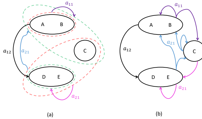
Figure 6: (a) A graph with a target node clustering (green dotted line) different from source node clustering (red dotted lines), only four connection coefficients are needed; (b) the corresponding SBM graph with a unique clustering and related constraints
