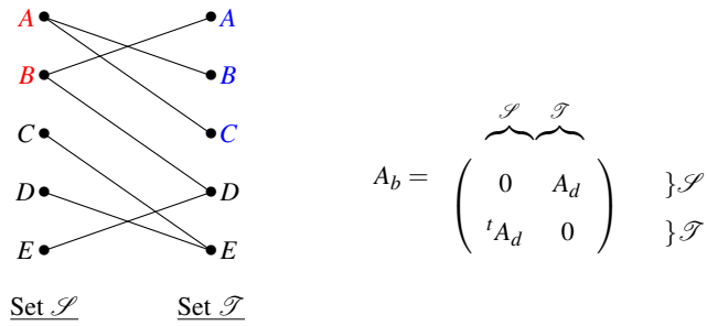
Figure 4: Directed graph of Figure 2 represented as a bipartite network between nodes with source and target roles on the left, with the corresponding adjacency matrix on the right.
