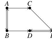
Figure 2: Directed graph.
