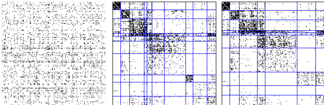
Figure 11: Enron dataset: original data (left), reorganized according to SBM with K = 10 node clusters (middle); co-clustering with H = 10 classes of emitters (rows) and 7 classes of receivers (columns).
