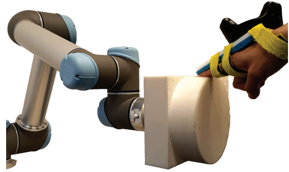
Fig. 8. Experimental setup. The hand support used for fixing the users' hand position and for sustaining the Vive tracker (upper right) and the multi-sided experimental prop with a flat surface integrated (center) this experimental prop was displaced and rotated by a robot unit (left) for having an ETHD-based approach.
