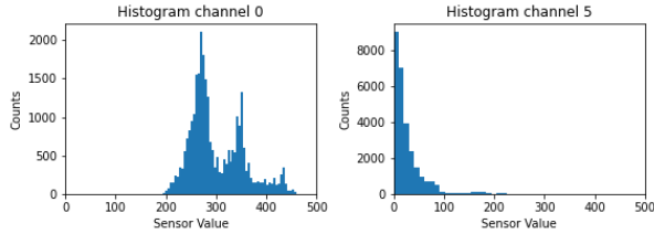
Figure 4: Histograms of two different textile sensors illustrating different conductive properties and how they relate to sensor responses to different movements. Left: Histogram of sensor 1 shows pronounced peaks for different movement types; the sensor captures a wide dynamic range of values. Sensor 6 shows very different properties, with most values being close to zero and some few large values.
