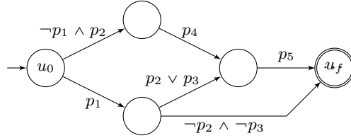
Fig. 2. A DD for formula (\neg p_1 \wedge p_2 \wedge p_4 \wedge p_5) \vee (p_1 \wedge (p_2 \vee p_3) \wedge p_5) \vee (p_1 \wedge \neg p_2 \wedge \neg p_3) .
