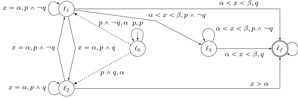
Fig. 1. A DTA specification of p\mathbf{U}^{\alpha, \beta}q with \alpha > 0 .
