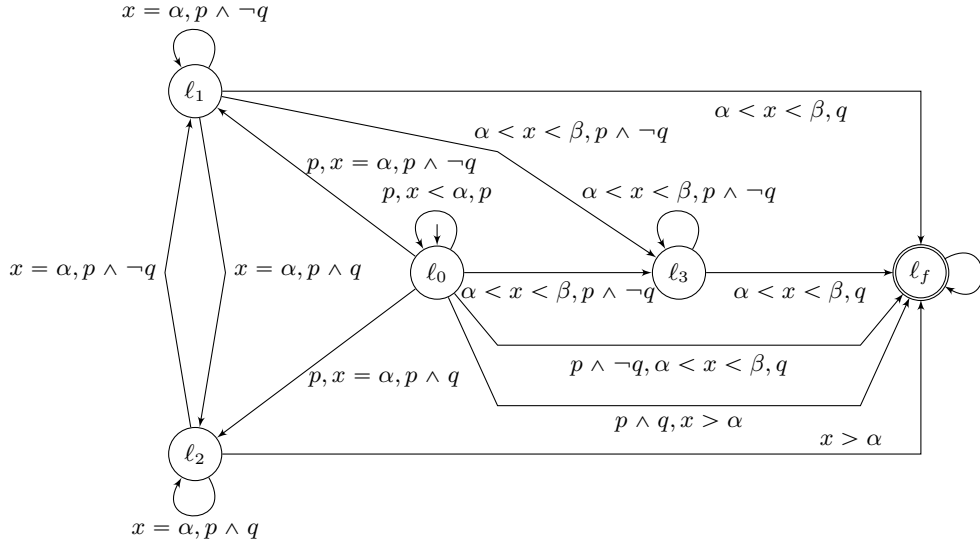
Fig. 3. Another DTA specification of p\mathbf{U}^{]\alpha, \beta[}q with \alpha > 0 .
