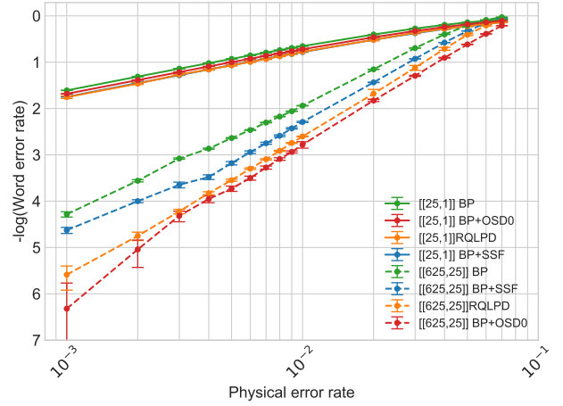
Fig. 5: Word error rate for several decoders on HPC starting from classical 3,4-regular random LDPC codes using independent X-type errors as noise model.
