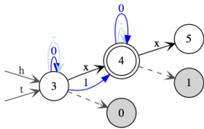
Figure 24. A single x -marked position.
