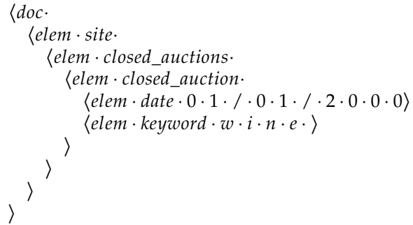
Figure 3. The corresponding nested word.
