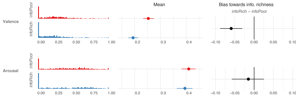
Figure 11: Raw responses, mean responses, and effect size in experiment 2, with 95% CIs.
