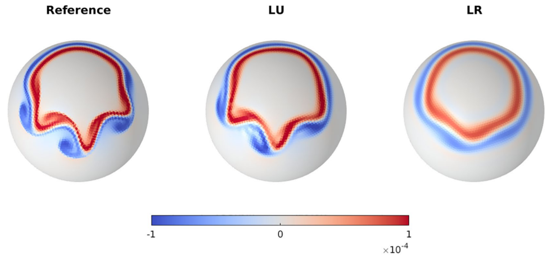
Figure 6. Snapshots of the vorticity field on the sphere for different models (with 20,480 triangles) after 5 days. From left to right: reference, ensemble mean of LU online and deterministic LR. For the simulations we use the parameters given in Table 1.
