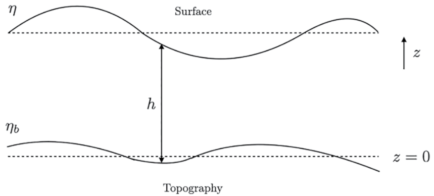
Figure 1. Illustration of a single-layered shallow water system (inspired by Vallis, 2017). h is the thickness of a water column, \eta is the height of the free surface and \eta_b is the height of the bottom topography. As a result, we have h = \eta - \eta_b .
