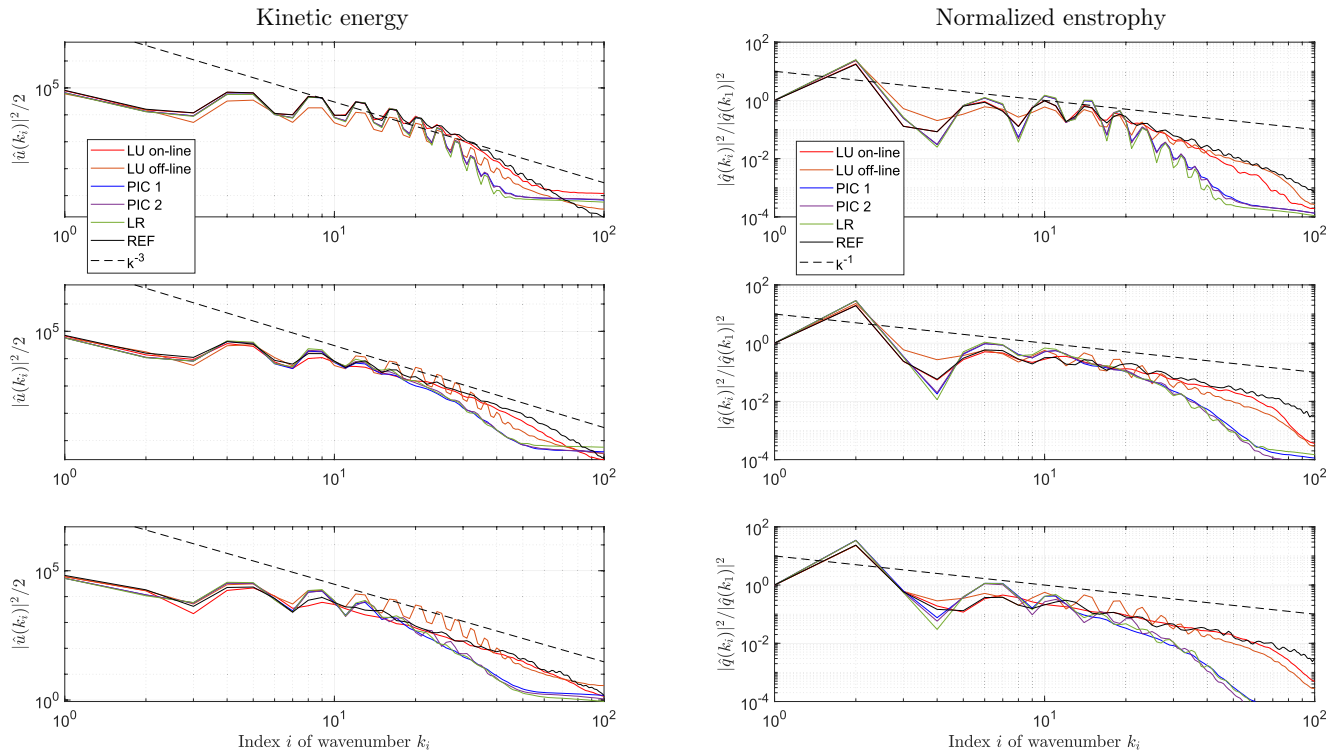
Figure 8. Comparison of the ensemble mean of the kinetic energy (left column) spectra and the potential enstrophy (right column) spectra for different models (with 20,480 triangles) at day 5 (1st row), 7 (2nd row) and 10 (3rd row) respectively. Note that the potential enstrophy is defined by the square of the potential vorticity and each potential enstrophy spectrum is normalized by its first value at the largest wavenumber. The dashed line is the k^{-3} (left column) and k^{-1} (right column) power law. These power laws for the RSW equations are discussed in (Chen et al., 2011; Ringler & Randall, 2002).
