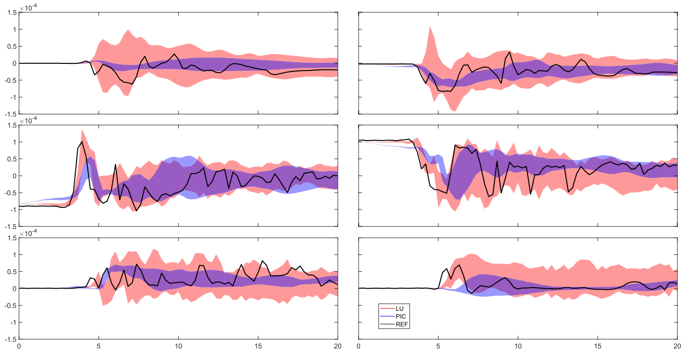
Figure 9. Comparison of the ensemble spread evolution over 20 days of the vorticity field for the LU-offline (red area) runs and the PIC-offline (blue area) runs, at six different locations \Theta = (0.4, 0.56, 0.72, 0.88, 1.04, 1.2) rad along the longitude Y = -1.53 rad. The observation trajectories are shown by the black lines.
