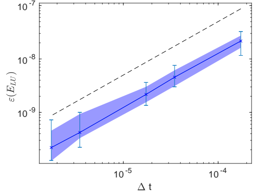
(b) Convergence of the energy path of the RSW-LU to that of the reference w.r.t. time step sizes. The blue line shows the global errors of the ensemble mean energy, the blue area describes the 68% confident interval of the ensemble errors and the dashed line stands for the 1st order convergence rate.
