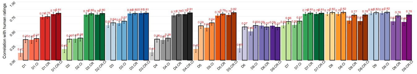
Figure 12: Performance, in terms of Pearson and Spearman correlation with mean opinion scores (MOS), of tested L_p -based BRDF metrics. For each metric D_i , we present its four variations. Cl stands for Clamping and CR stands for Cubic Root. Bars without border refer to Pearson and bars with black borders refer to Spearman. The error bars indicate the 95% intervals computed by bootstrapping.
