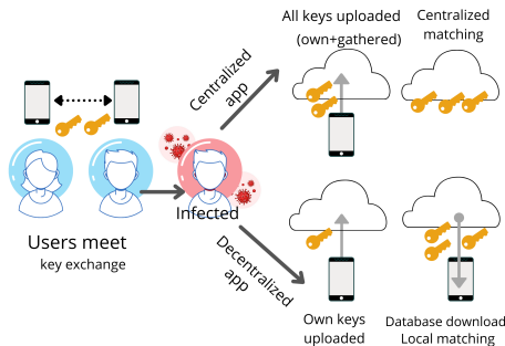
Figure 1: Centralized vs Decentralized bluetooth-based apps
