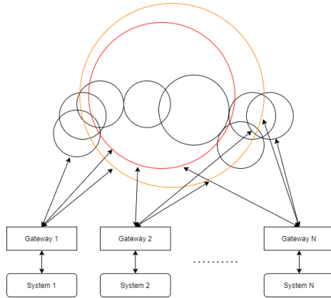
Figure 3: BAC19 Federation Overlay Network
