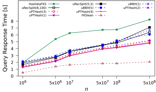
Figure 5 – The response time for 10^7 queries, in seconds, of all methods on the random hypergraphs. The x-axis is in log-scale. At n = 5 \times 10^8 , the plots correspond to, from top to bottom, the methods as listed in the legend (from left to right, top to bottom).
