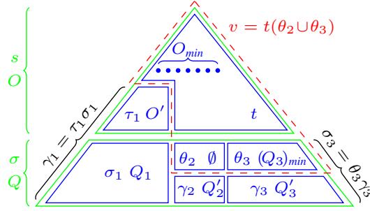
Figure 1: Proof of Lemma 27 with P' \neq \emptyset .
