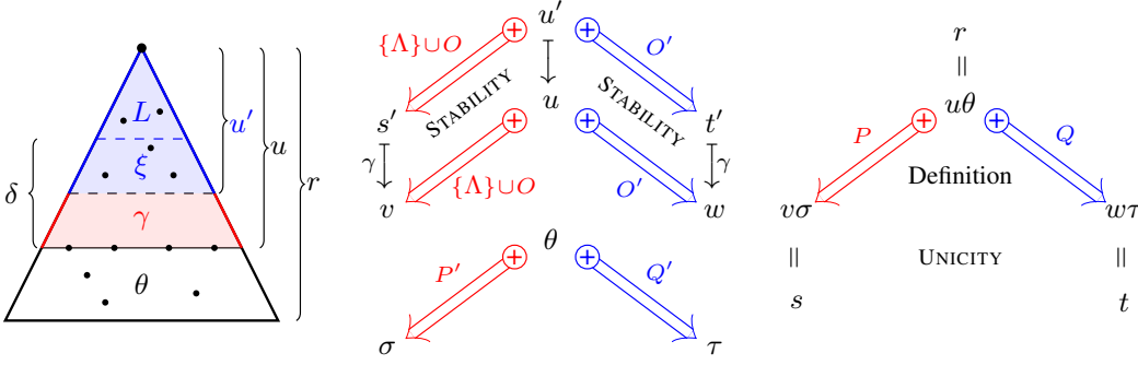
Figure 3: Nested critical peak property
