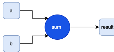
Figure 1: The operation c = a + b represented as a TensorFlow graph.
