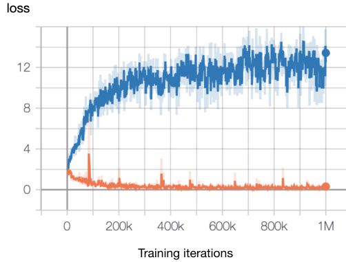
Figure 21: GCT with hyperparameters of the approach CXL+19 : Loss on the validation set (blue) and loss on the train set (orange) during training.
