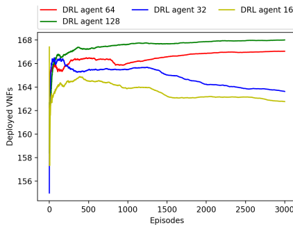
Fig. 3. Number of accepted VNFs vs Number of hidden units.
