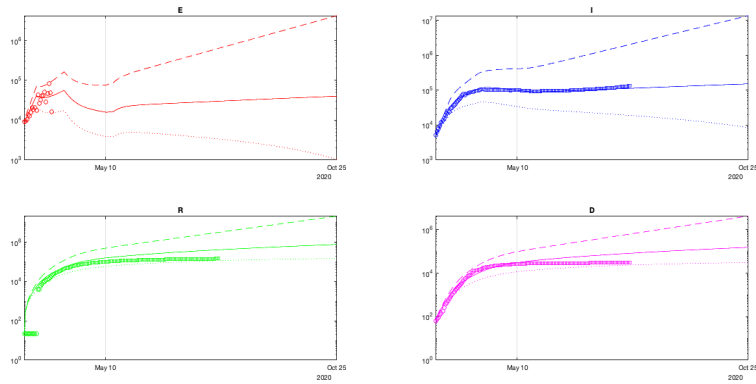
Figure 6: The results of simulation of (9) for France under \pm 7.5\% variation of all parameters
