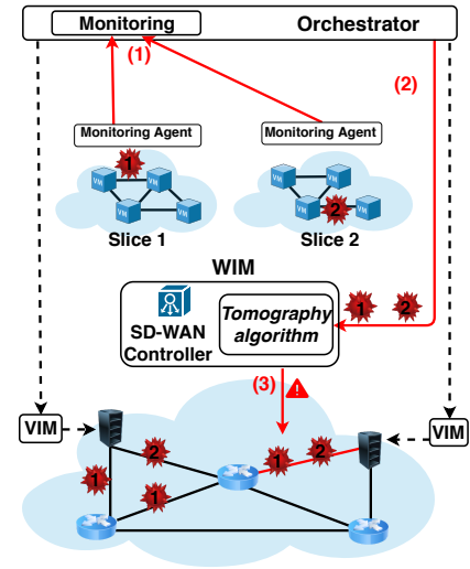
Fig. 1: Slices monitoring
