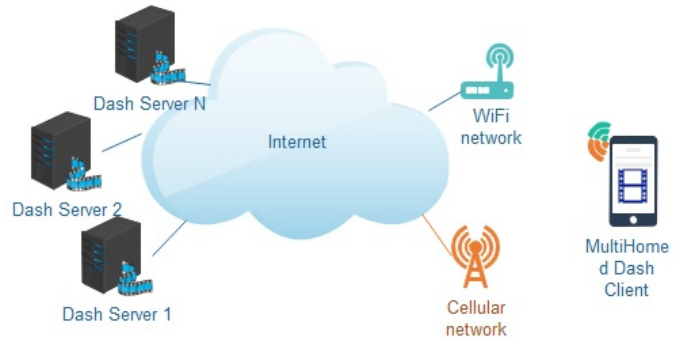
Fig. 1. Multihoming Infrastructure
