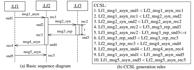
Fig. 1. Transformation of basic sequence diagram
