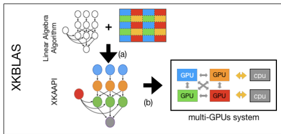
Fig. 2. Overview of XKBlas/XKaaapi steps.
