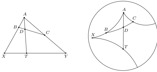
Fig. 5: Tarski's parallel postulate A10.
